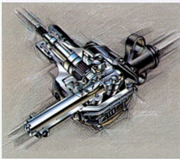
The Prelude Si 4WS has a second steering gear to control the rear wheels.
